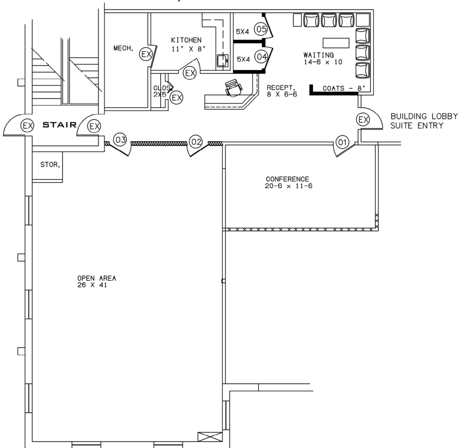
PARTIAL FIRST FLOOR PLAN
