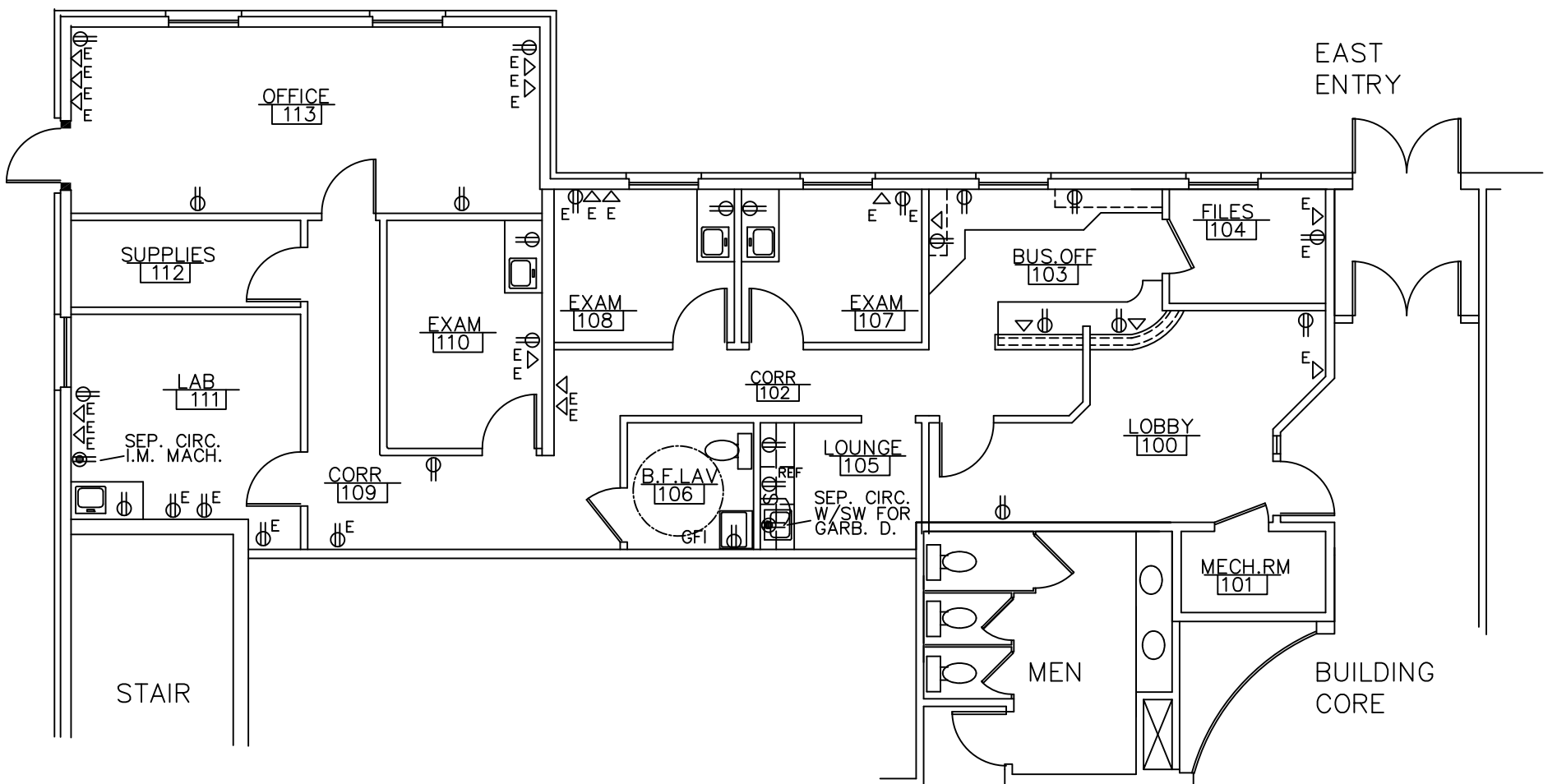
PARTIAL FIRST FLOOR ELECT./COMM. PLAN SCALE: 1/4" = 1'-0"
